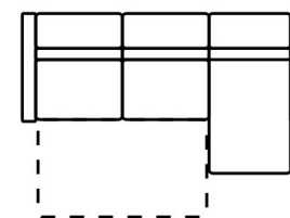
BW1L-3RF0-1,5SWP 276 / 126-172 / h 48-82-101 incl. feet 14 cm
